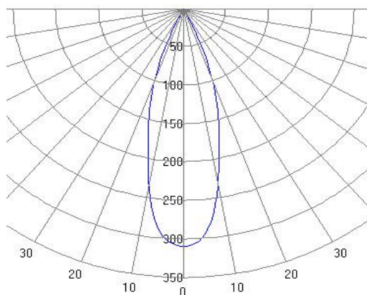
配光曲线-极坐标 Light distribution curve-polar coordinates
