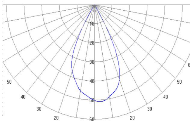
配光曲线-极坐标 Light distribution curve-polar coordinates
