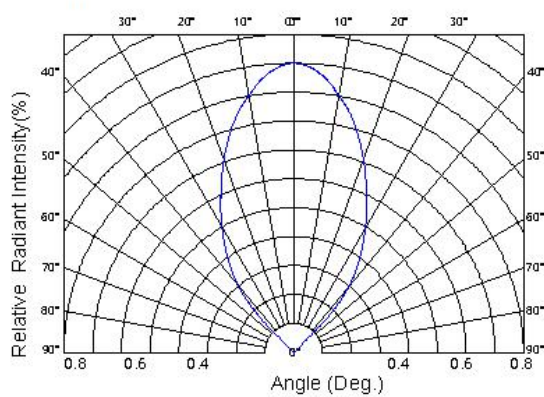
FIG:6 Radiant Intensity Spatial Distribution
