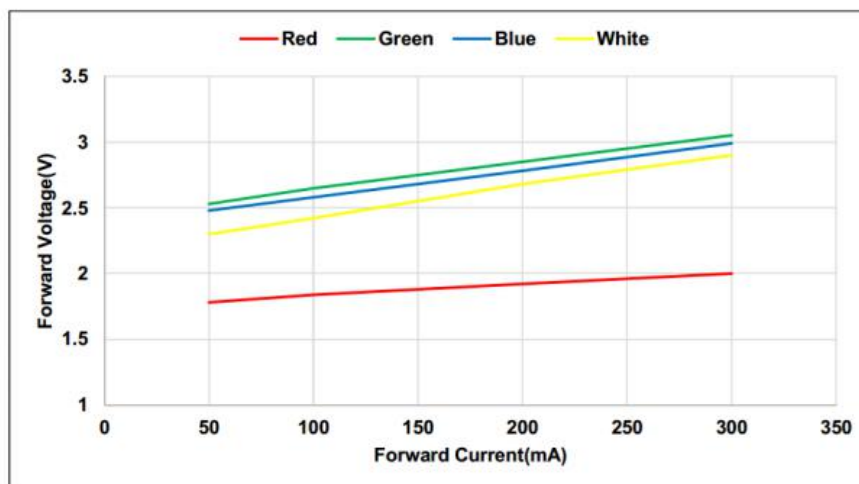
Fig 3. Forward Voltage vs. Forward Current , T_a = 25^\circ\text{C}
