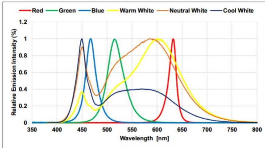
Fig 1. Color Spectrum, T_a = 25^\circ\text{C} , RH60%
