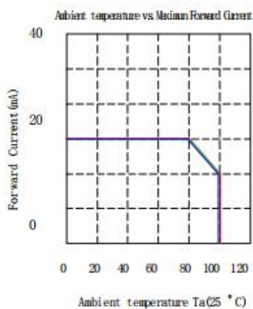
Derating
