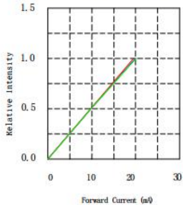
Relative Intensity vs. Forward Current ( T_a=25^\circ\text{C} )
