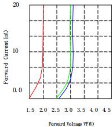
Forward current vs. Forward Voltage ( T_a=25^\circ\text{C} )
